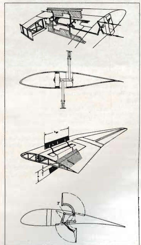
Fig 21. Airbrakes: a) Vertical movement top and bottom airbrakes. The brake caps lie flush with the wing surface. b) Rotating top and bottom airbrakes where the whole brake surface lies flush with the wing surface. On opening, the lower brake helps pull out the top surface brake.
