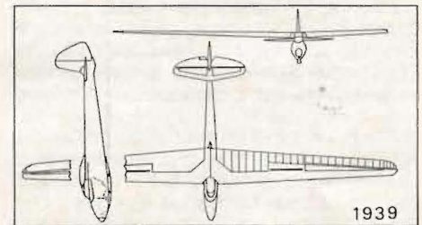
Fig 27. The outstanding 15m Meise Olympia.
