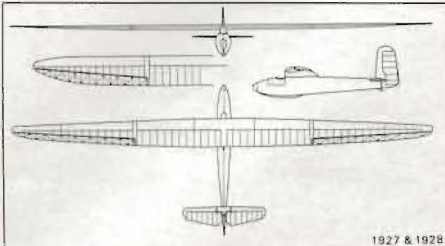
Fig 6. The 16m Darmstadt 1 and the 18m Darmstadt 2.
